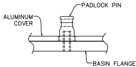
DETAILED SIDE VIEW OF PADLOCK PIN INSTALLED
