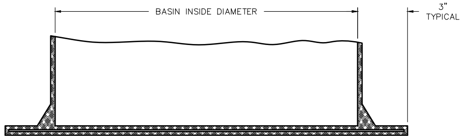
BOTTOM ANTI-FLOATATION FLANGE
