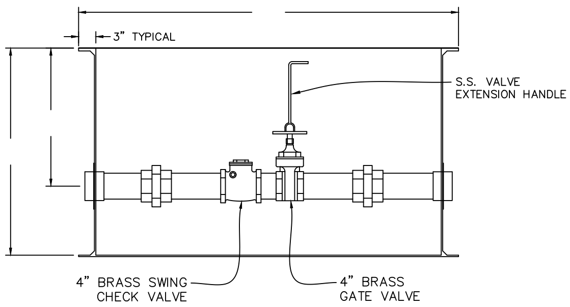
SECTIONAL ELEVATION VIEW
