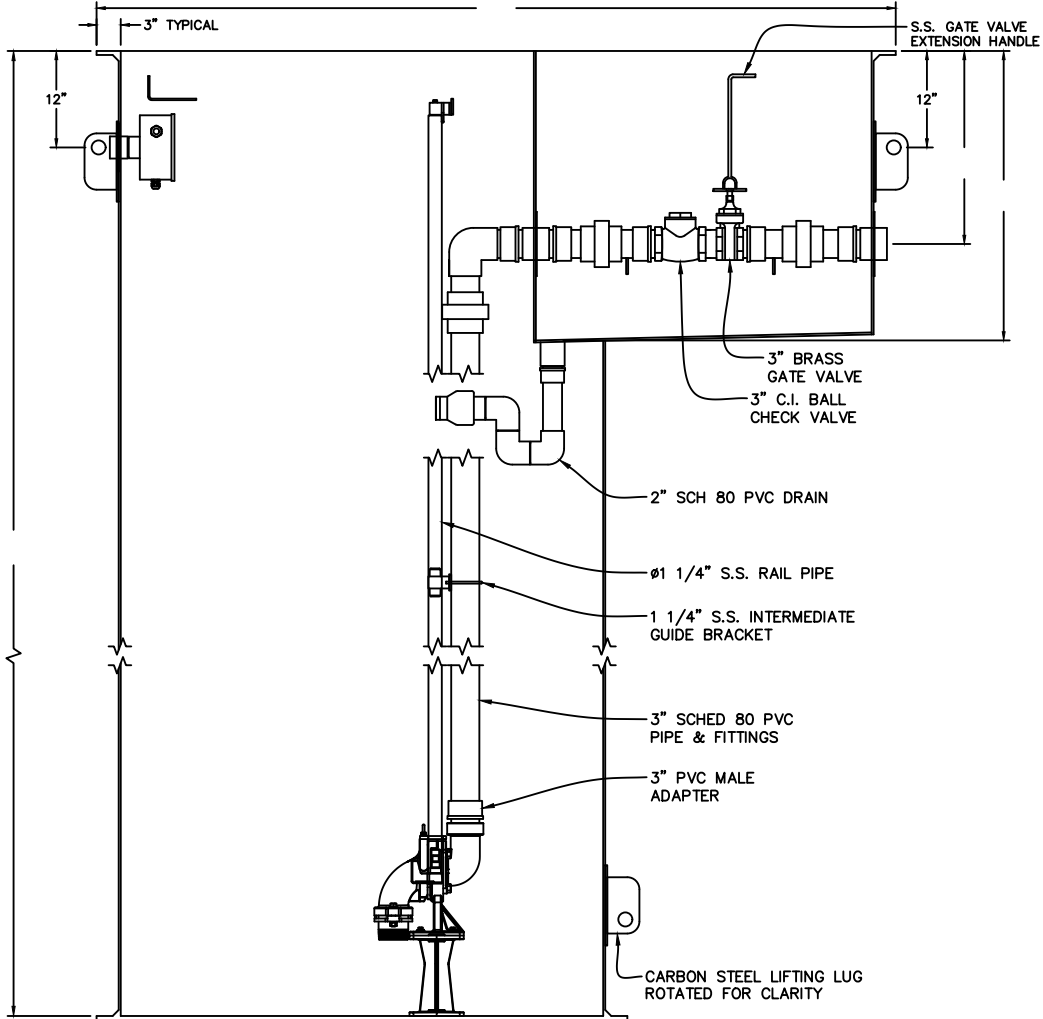
SECTIONAL ELEVATION VIEW
