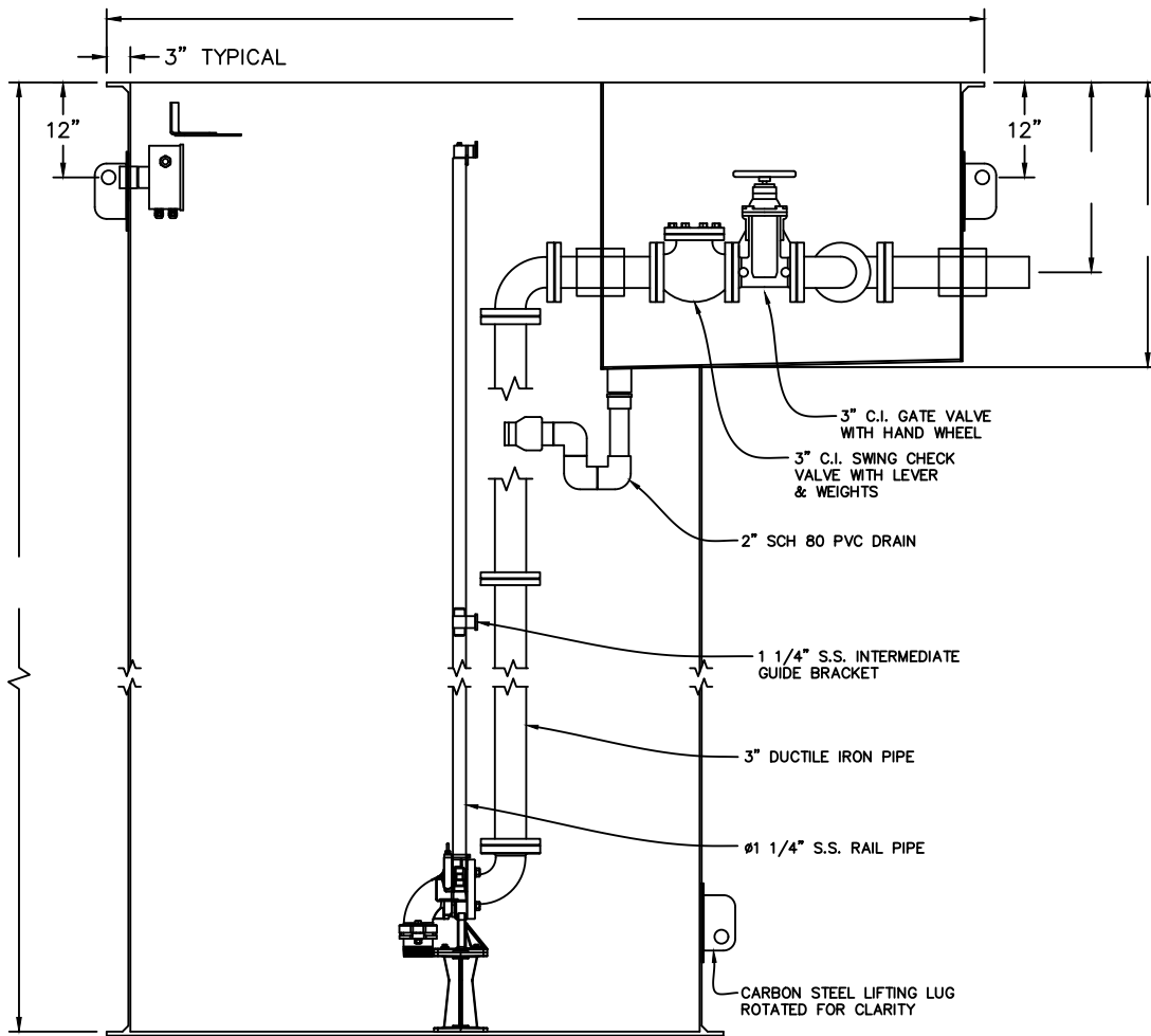
SECTIONAL ELEVATION VIEW
