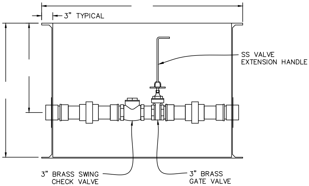
SECTIONAL ELEVATION VIEW
