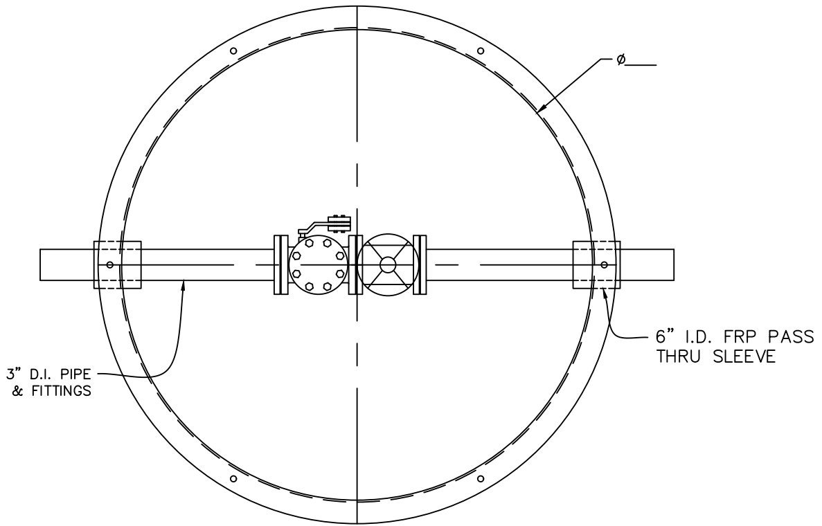
PLAN VIEW
