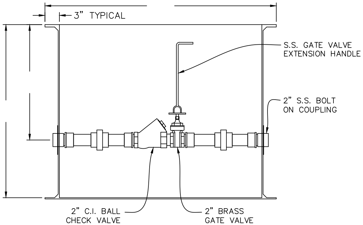
SECTIONAL ELEVATION VIEW
