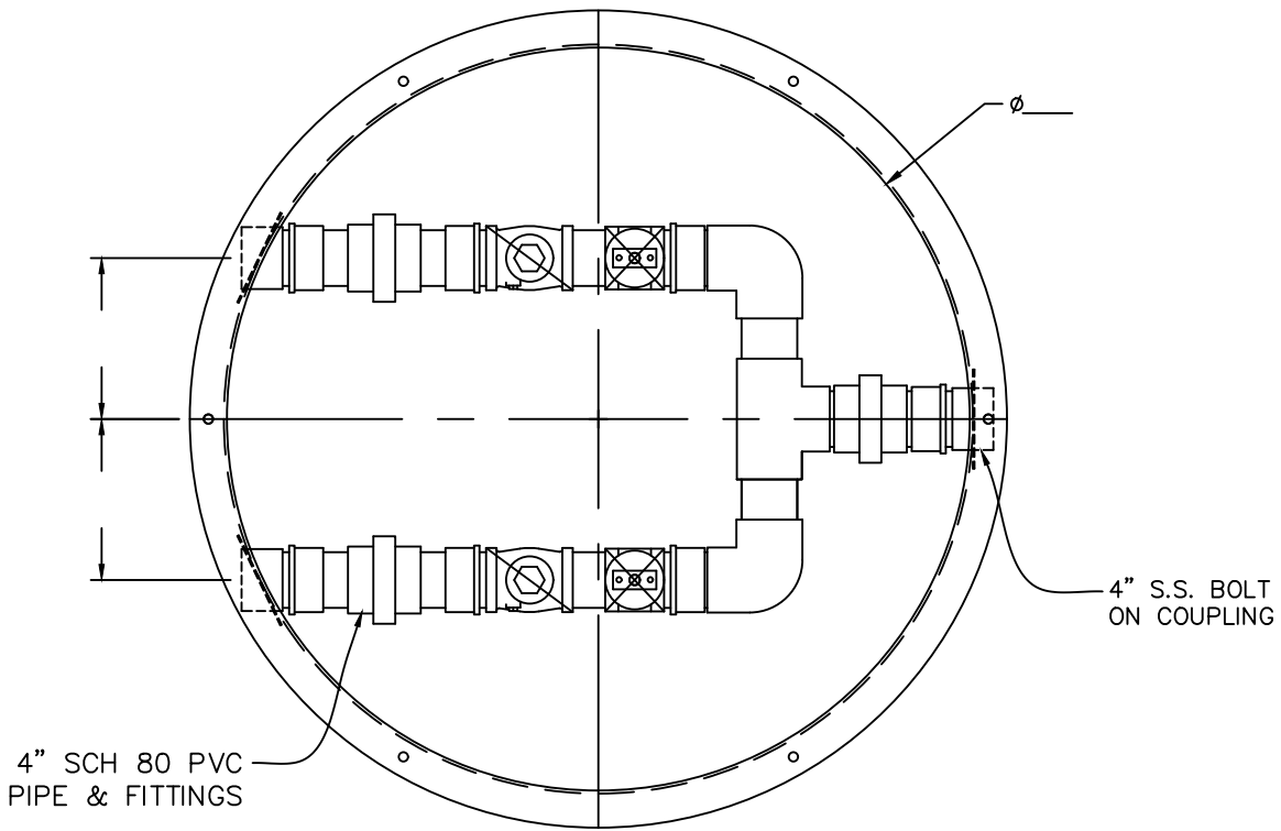
PLAN VIEW
