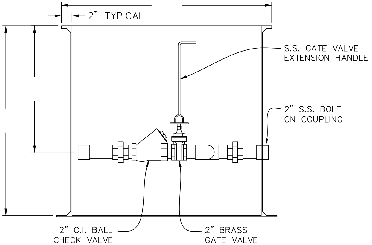
SECTIONAL ELEVATION VIEW
