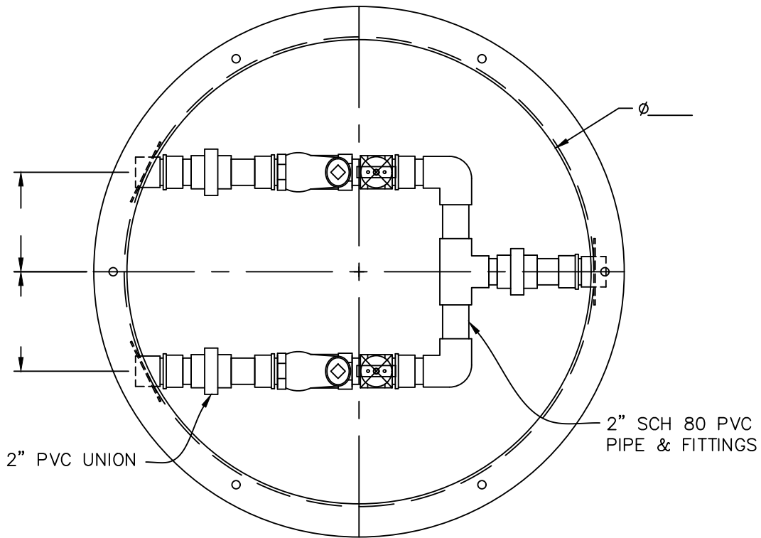
PLAN VIEW
