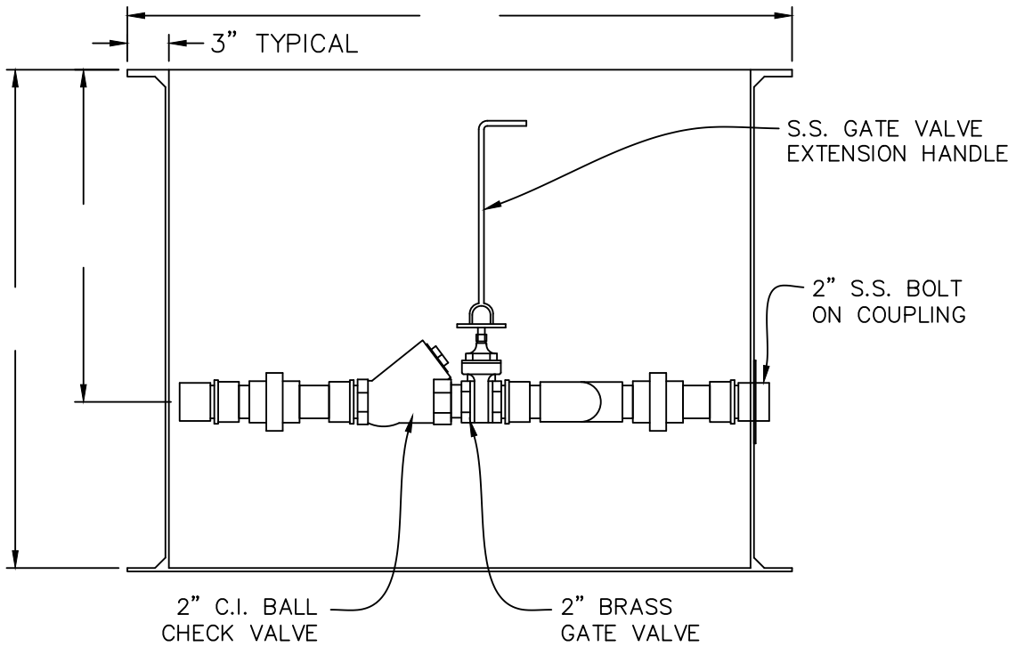
SECTIONAL ELEVATION VIEW
