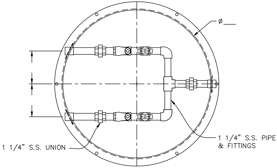
PLAN VIEW
