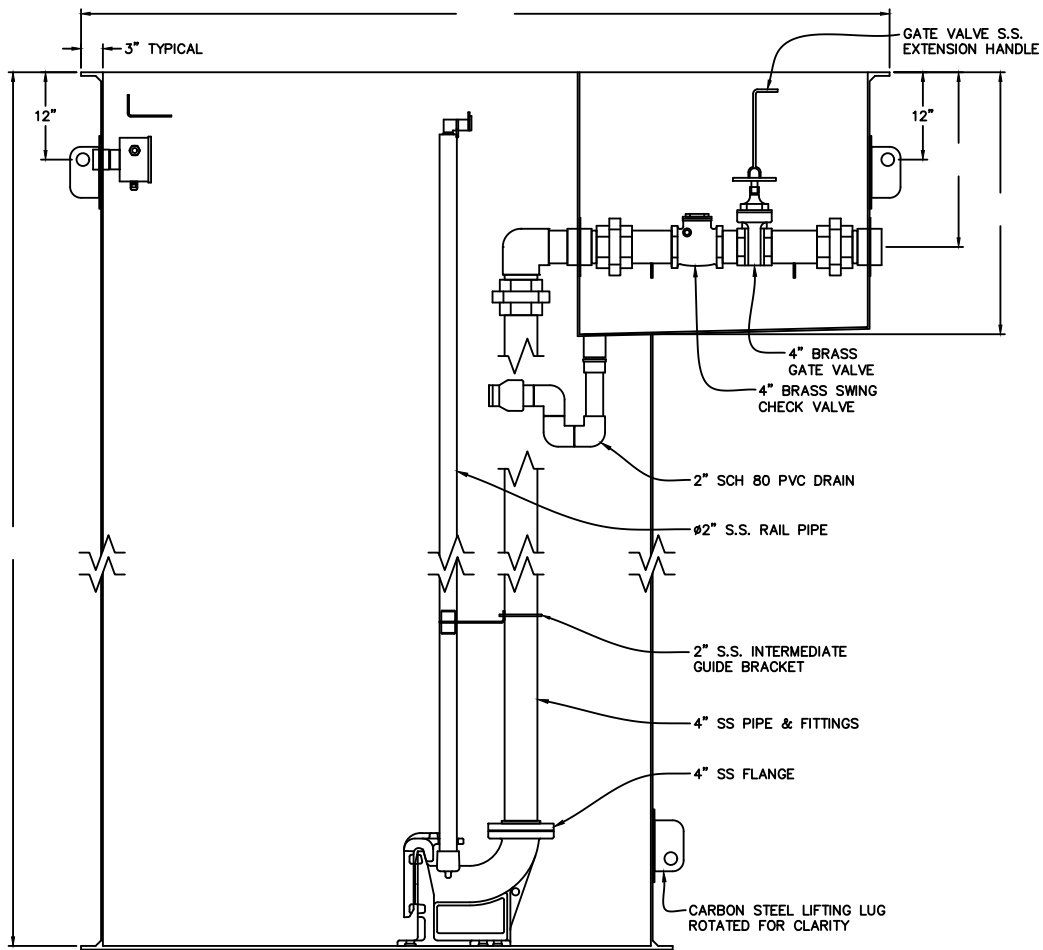
SECTIONAL ELEVATION VIEW
