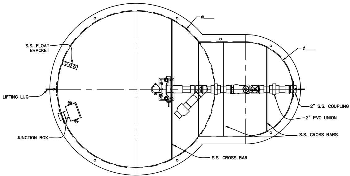
PLAN VIEW
