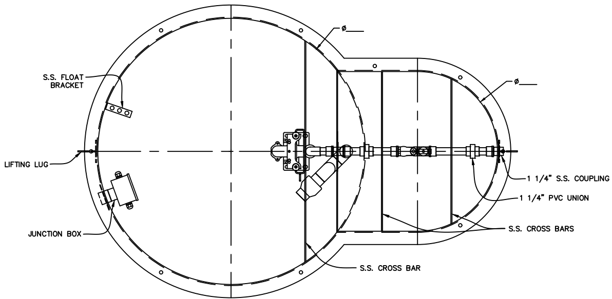
PLAN VIEW
