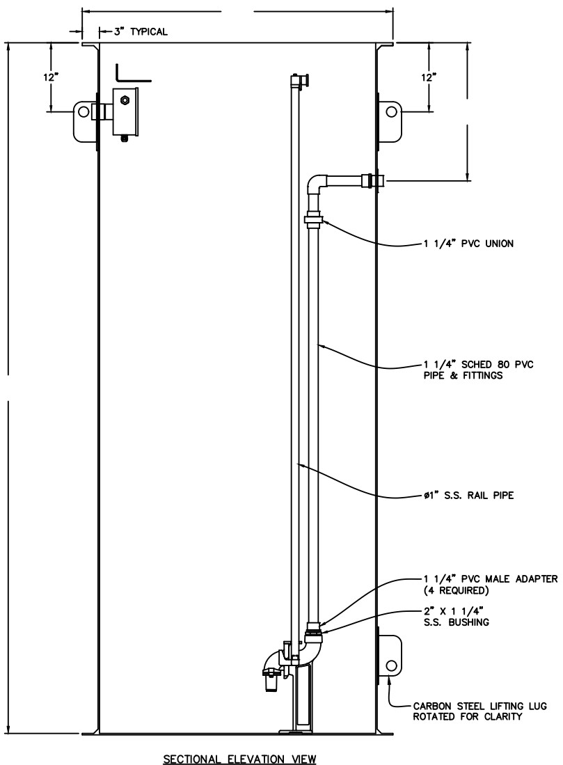
SECTIONAL ELEVATION VIEW
