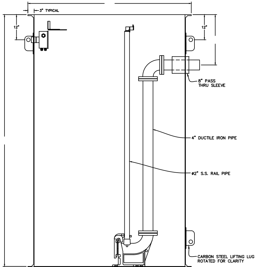
SECTIONAL ELEVATION VIEW
