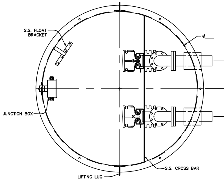
PLAN VIEW
