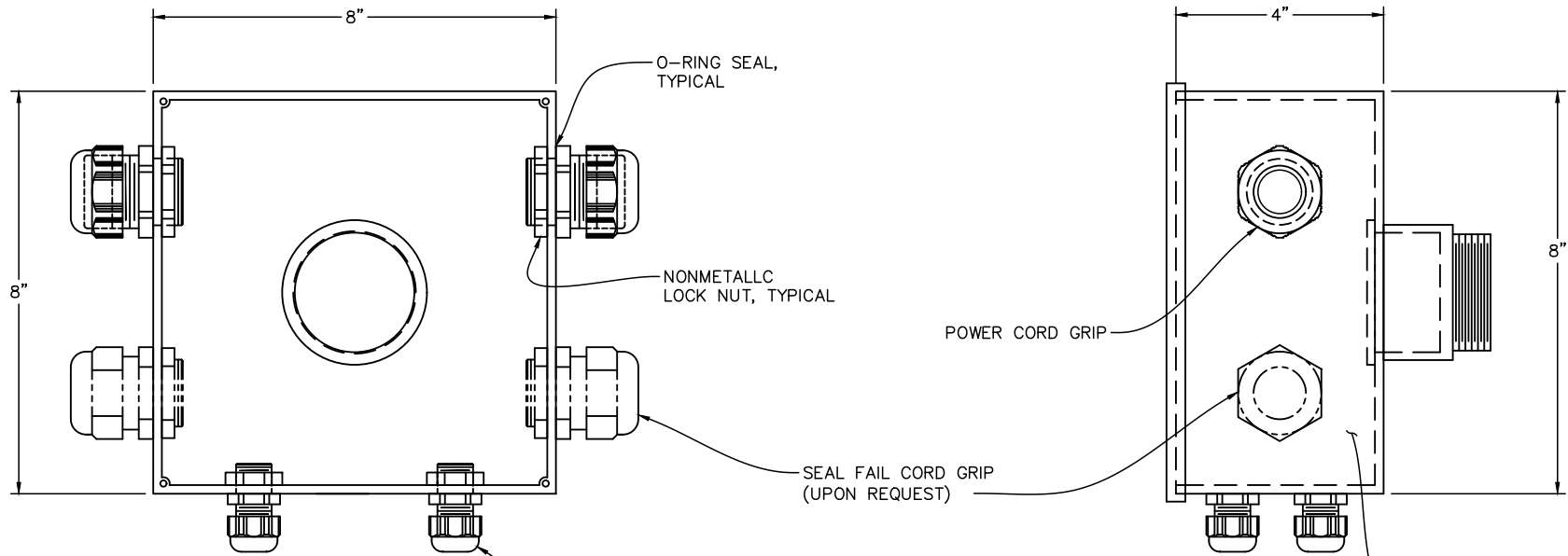
FRONT VIEW WITH COVER REMOVED
