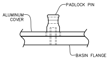
DETAILED SIDE VIEW OF PADLOCK PIN INSTALLED
