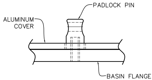
DETAILED SIDE VIEW OF PADLOCK PIN INSTALLED
