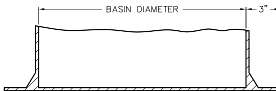
BOTTOM ANTI-FLOATATION FLANGE
